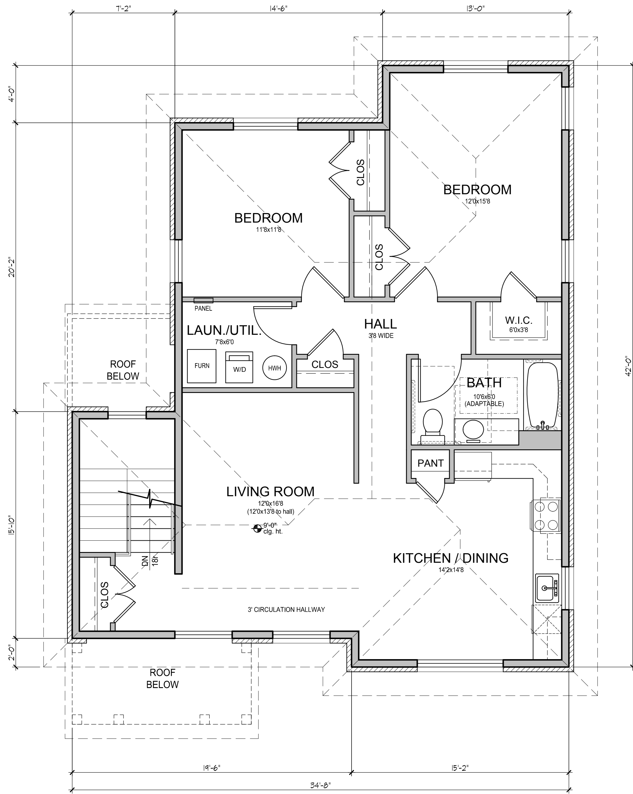
UPPER LEVEL UNIT SCALE: 1/4"=1'-0" UNIT AREA = 1,115 SQ FT
