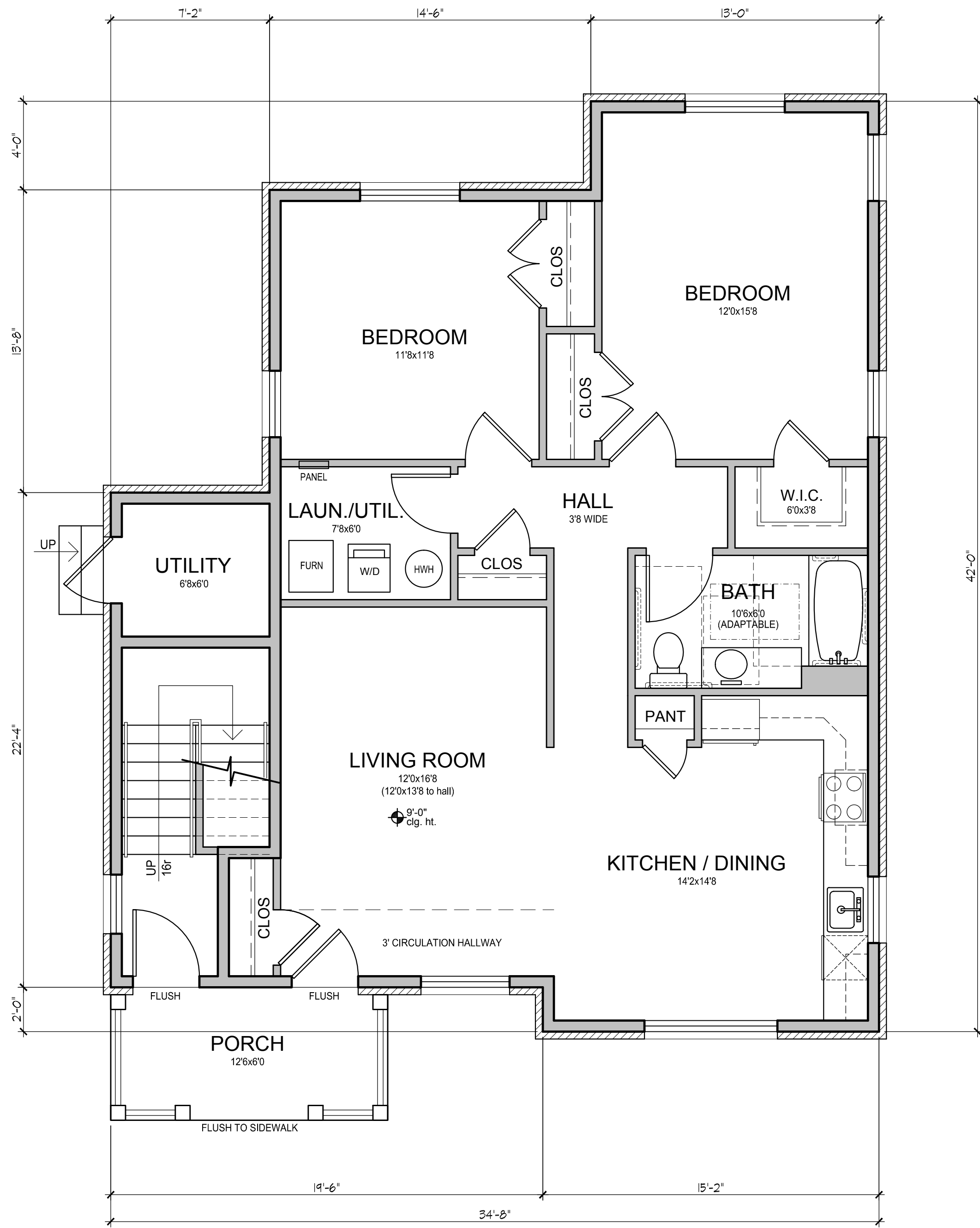
LOWER LEVEL UNIT SCALE: 1/4"=1'-0" UNIT AREA = 1,088 SQ FT
